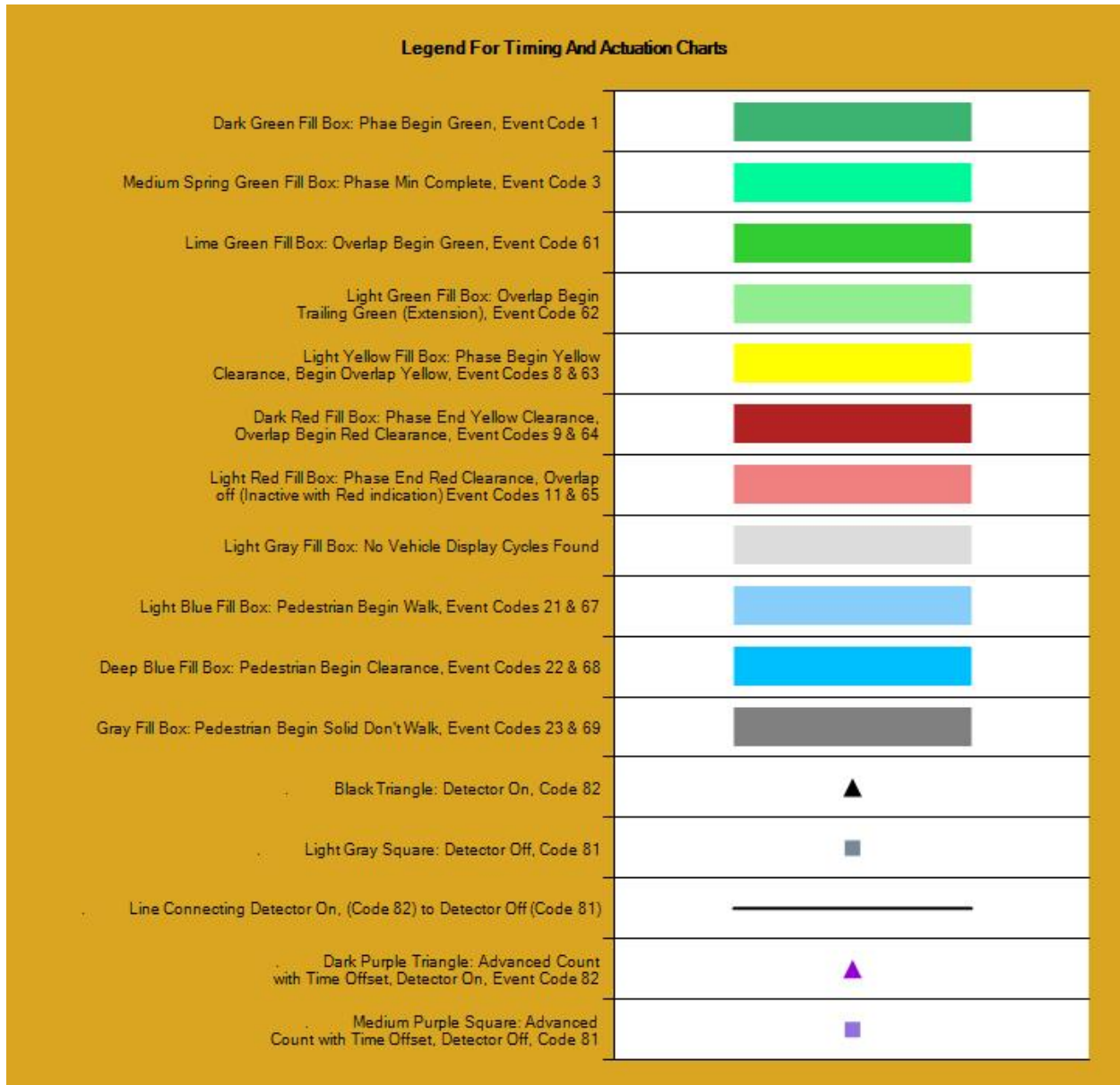
Figure 22: Legend for Timing and Actuation Charts
