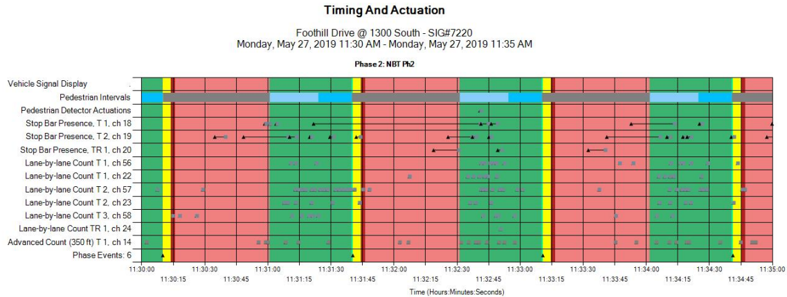
Figure 24: Timing and Actuation Chart - Phase Event Codes
