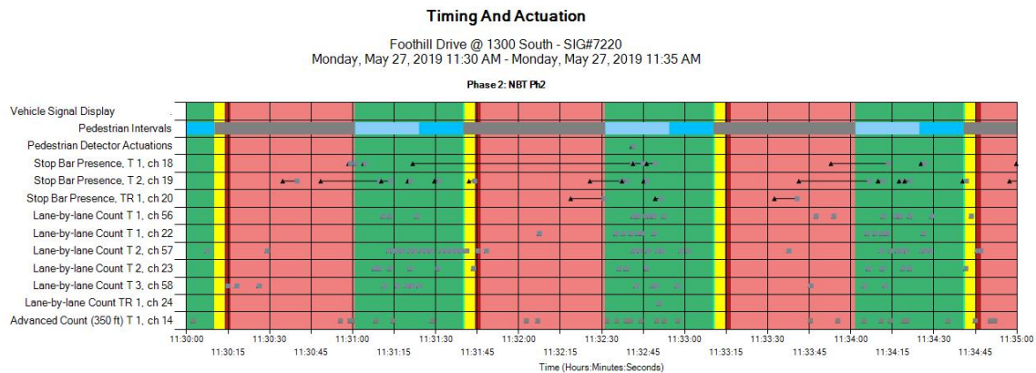
Figure 23: Timing and Actuation Chart
