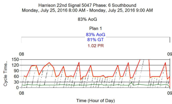
Figure 36: PCD (Existing & Predicted) for Purdue Link Pivot
